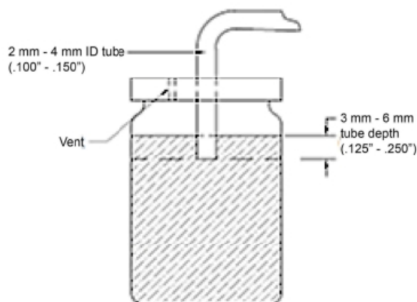
Figure 1—Volumetric Device
